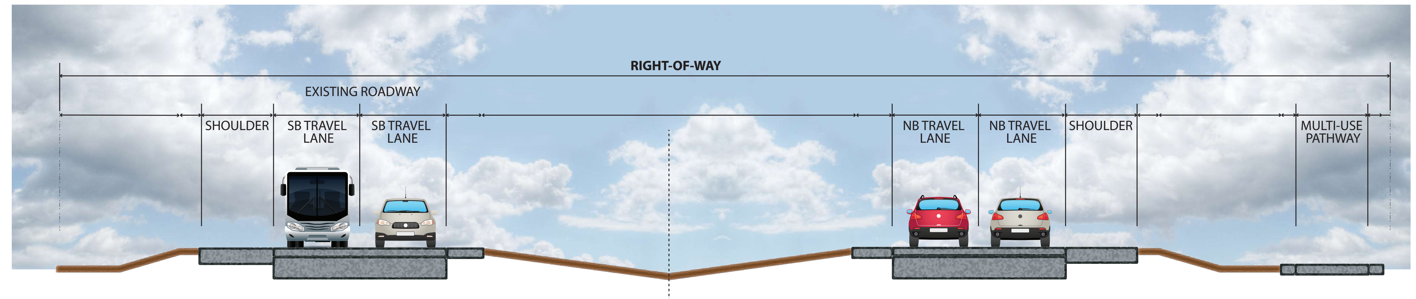
NORTH SEGMENT: Freeway, Alternatives A and B (Marsh Creek to Armstrong Road, typical)
