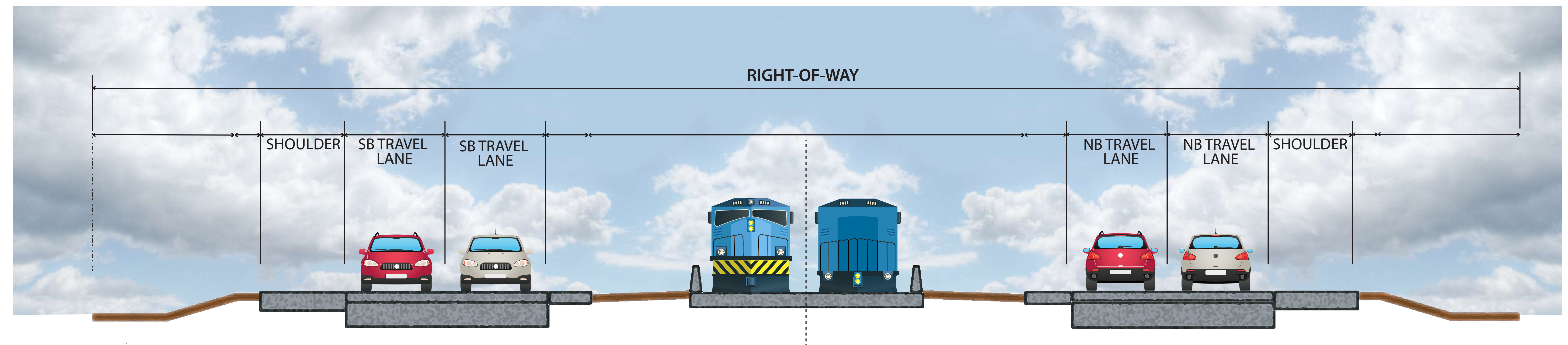
SOUTH SEGMENT: Freeway, Alternative A (Armstrong Road to Interstate 580, typical)
