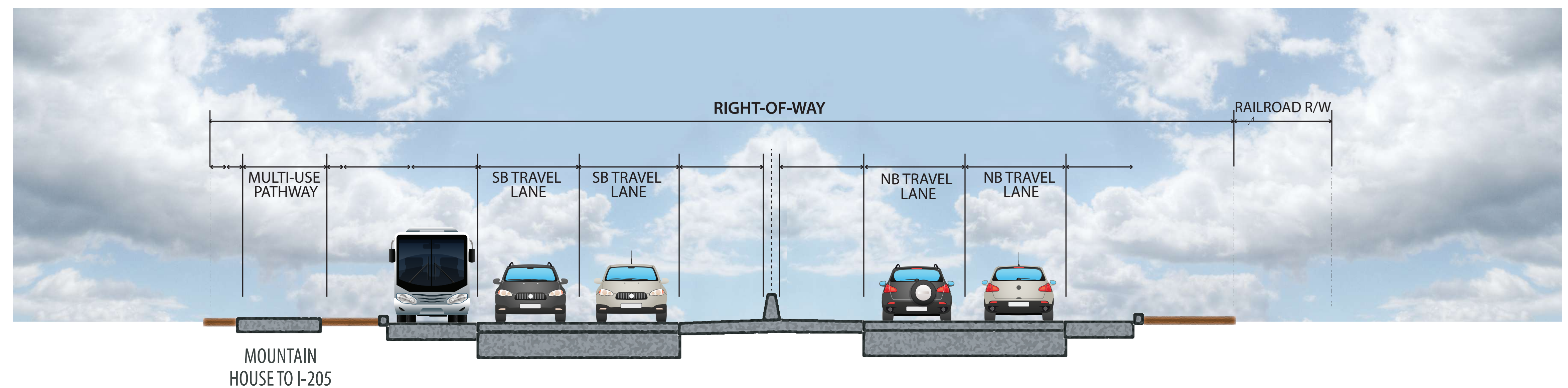
SOUTH SEGMENT: Expressway, Alternative B (Armstrong Road to Interstate 205)
