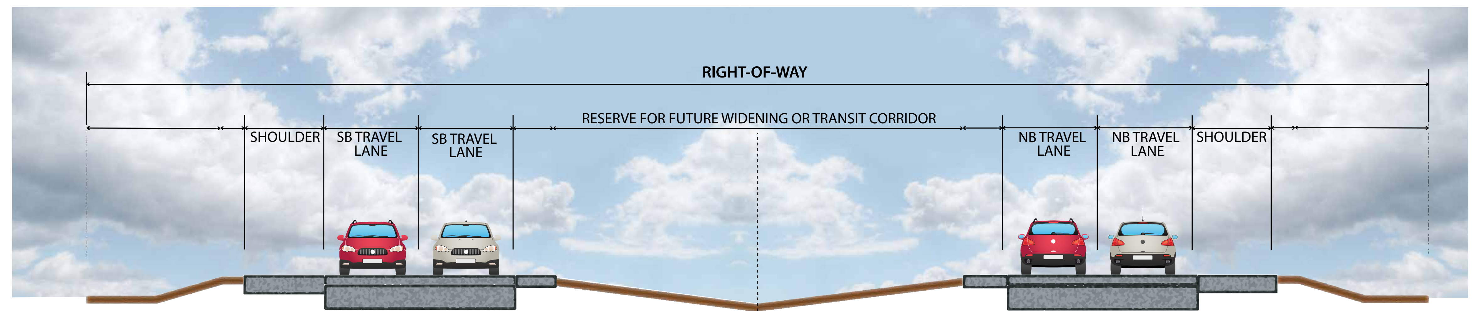
SOUTH SEGMENT: Freeway, Alternative A (Armstrong Road to Interstate 580, typical)
